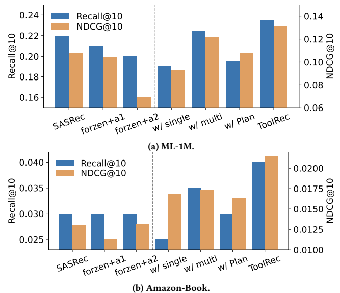
Figure 4: Performance of ToolRec and its variants. The right side of the dividing line indicating the methods involving LLMs.
